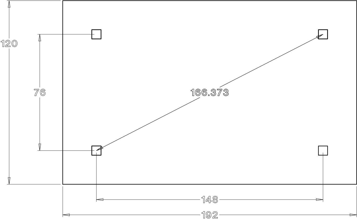
8 x 14 Vinyl pergola
